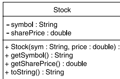
Figure 8-8 UML diagram for the Stock class
