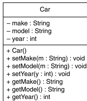
Figure 6-30 UML diagram for the Car class
