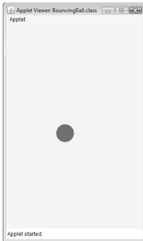
Figure 14-31 BouncingBall applet
