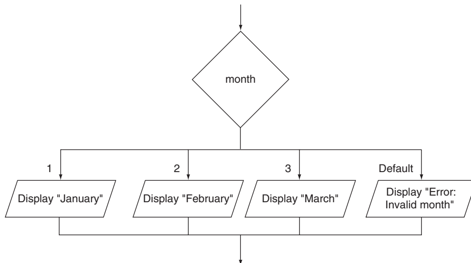
Figure 3-24 A multiple alternative decision structure
