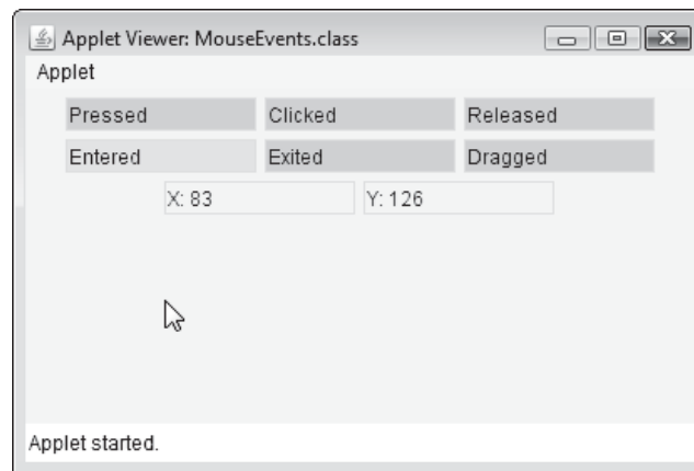
Figure 14-29 MouseEvents applet
